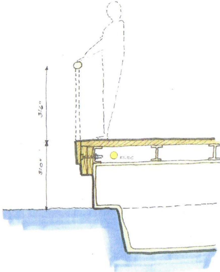
HARBOR SIDE SECTION NT6
