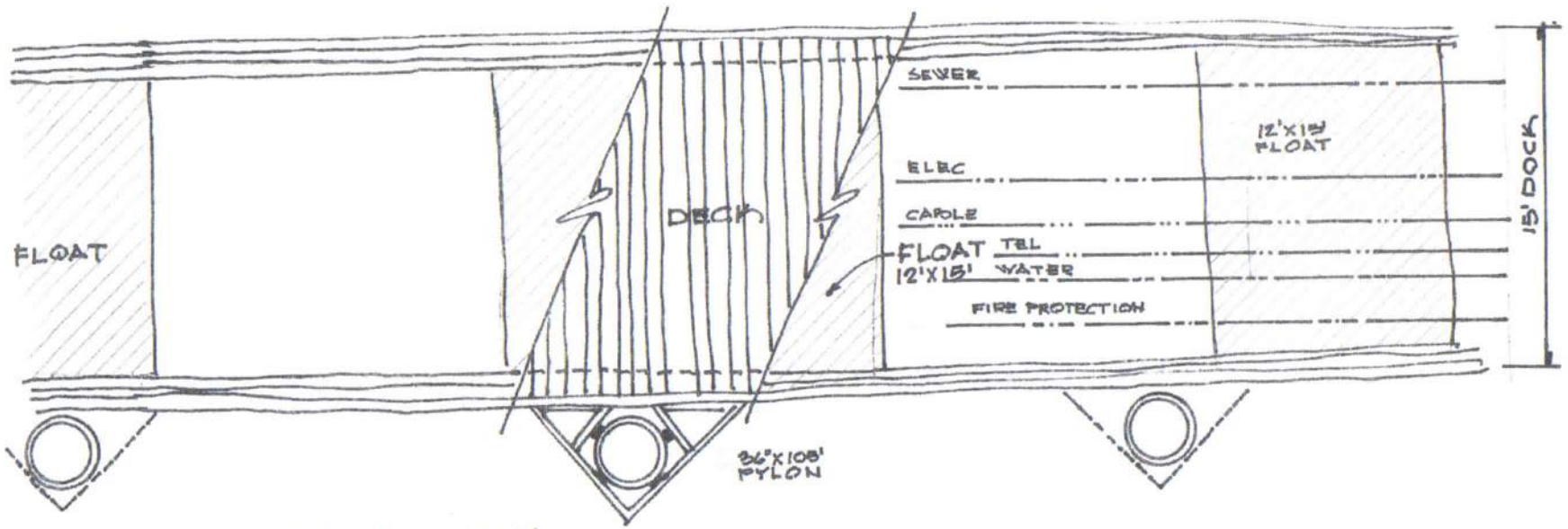
UTILITY DISTRIBUTION PLAN NTS
