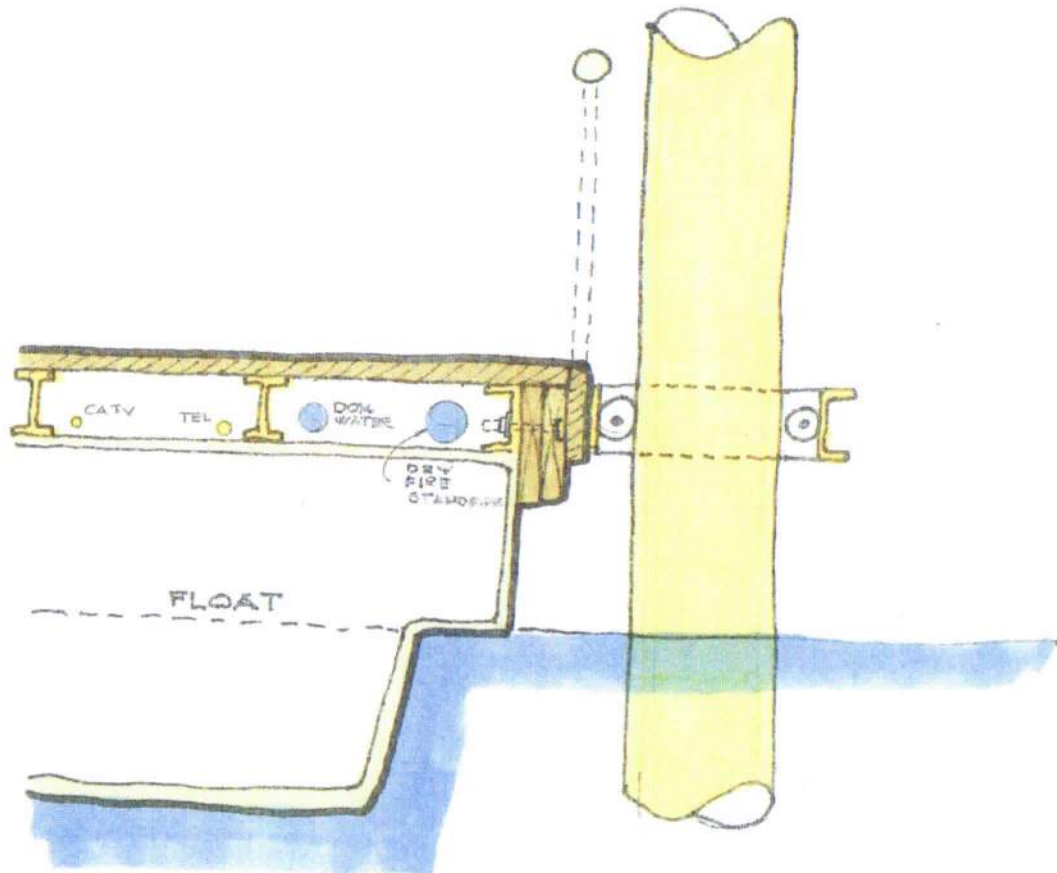
SHORE SIDE SECTION NT6
