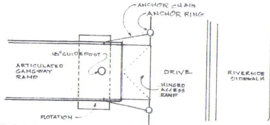
GANGWAY RAMP PLAN @ TOP
