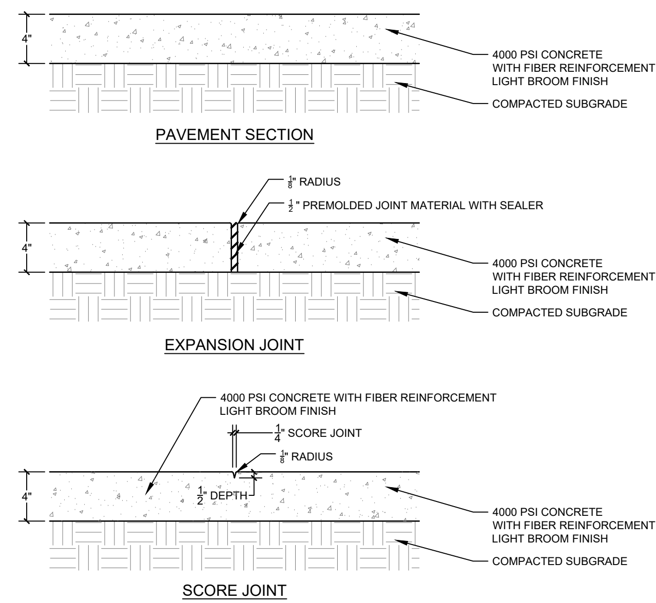
1 TYP. 4" CONCRETE SCALE: NTS
